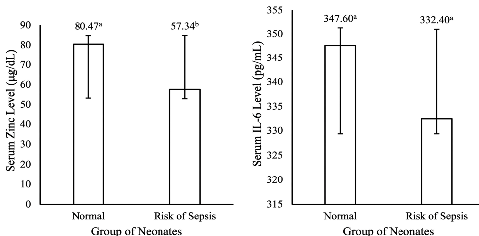
Fig. (1). Comparison of serum zinc and IL-6 levels in normal and at-risk-of-sepsis neonates. Data presented as mean \pm SD. Different lowercase letter p < 0.001 for zinc levels between groups. Different lowercase letters indicate statistically significant differences between normal and at-risk-of-sepsis neonates ( p < 0.05 ).
